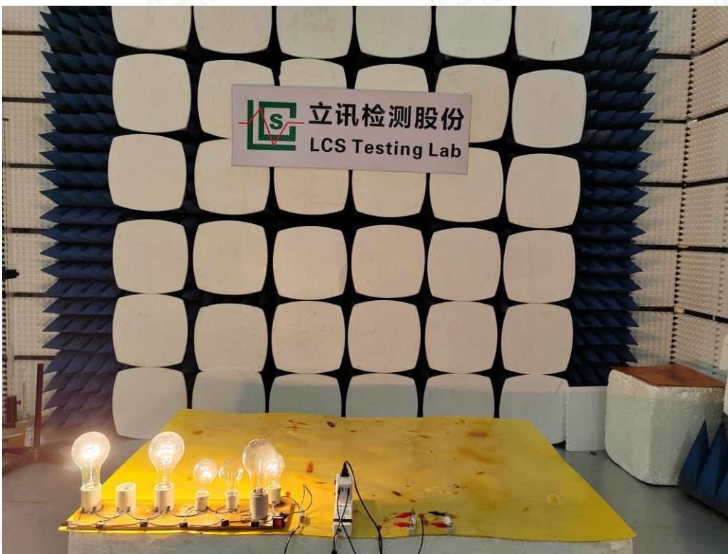
Test Setup Photo of RF Field Strength Susceptibility
