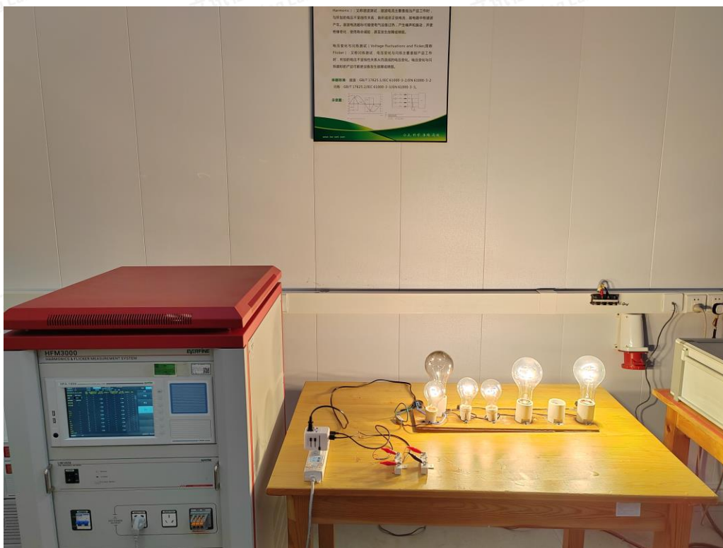
Test Setup Photo of Harmonic & Flicker Measurement
